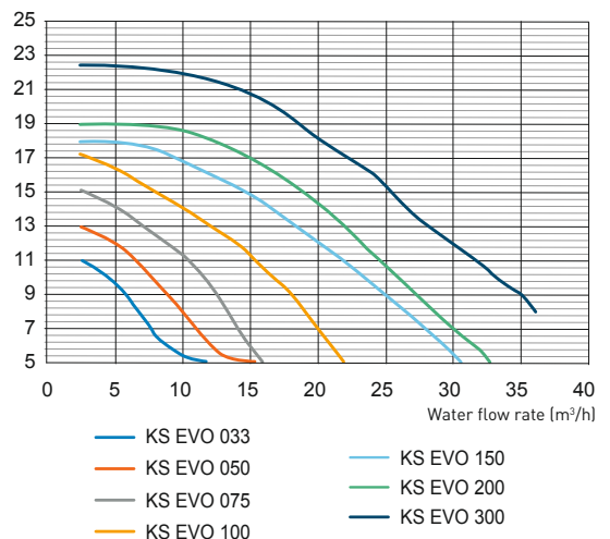
Water column pressure (m) KS Evo / KSX Pro Q (m 3 /h)-H (m)
